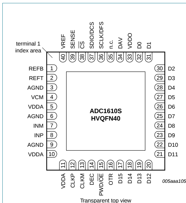
Fig 2. Pin configuration with CMOS digital outputs selected
