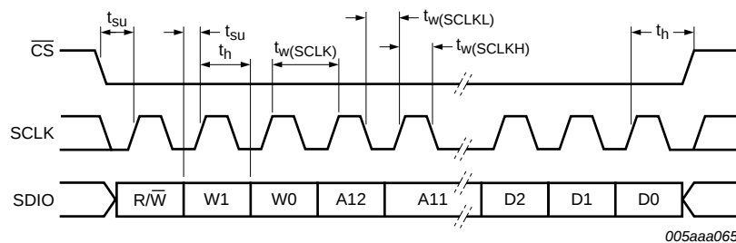
Fig 6. SPI timing
