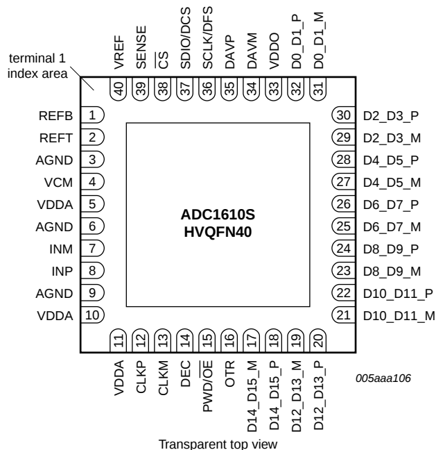
Fig 3. Pin configuration with LVDS DDR digital outputs selected
