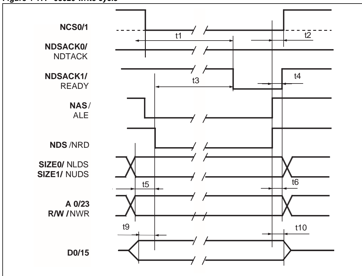
Figure 4-17: 68020 write cycle
