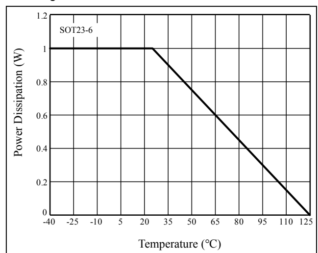
Figure 35 P_D vs. T_A (SOT23-6)
