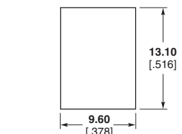
Recommended Panel Cutout Max. Panel Thk. 1.7 [.067]
