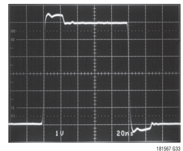
Large-Signal Transient, A_V = 1 , V_S = \pm 5V
