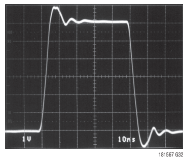
Large-Signal Transient, A_V = -1 , V_S = \pm 5V
