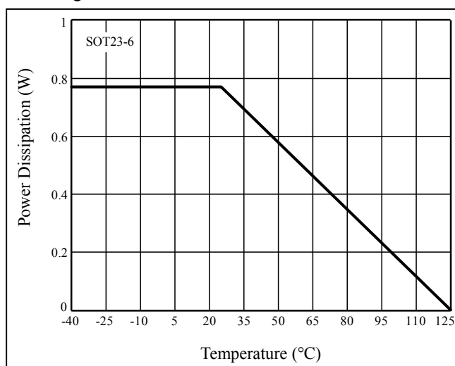
Figure 35 P_D vs. T_A (SOT23-6)
