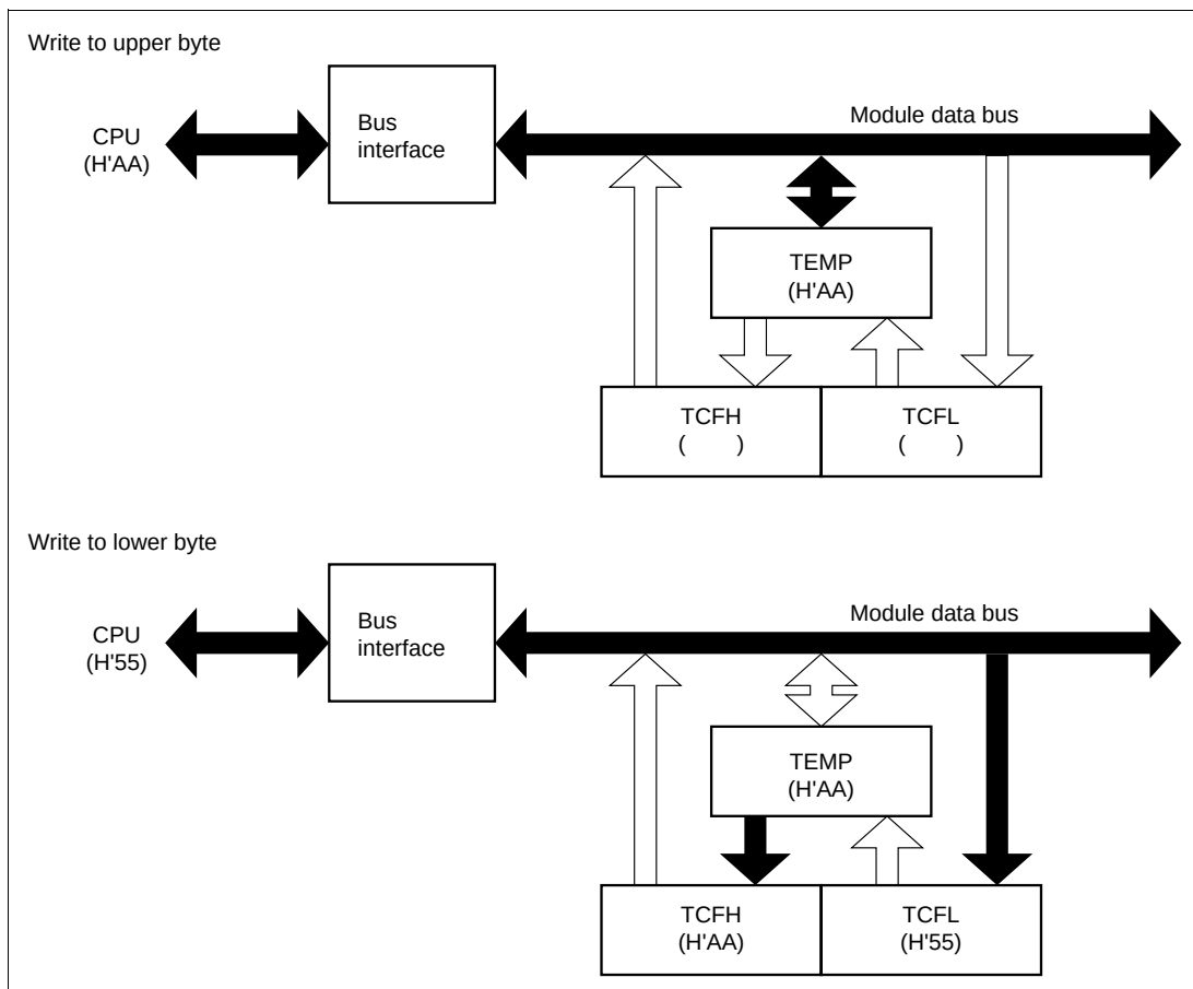
Figure 9.4 Write Access to TCF (CPU Æ TCF)
