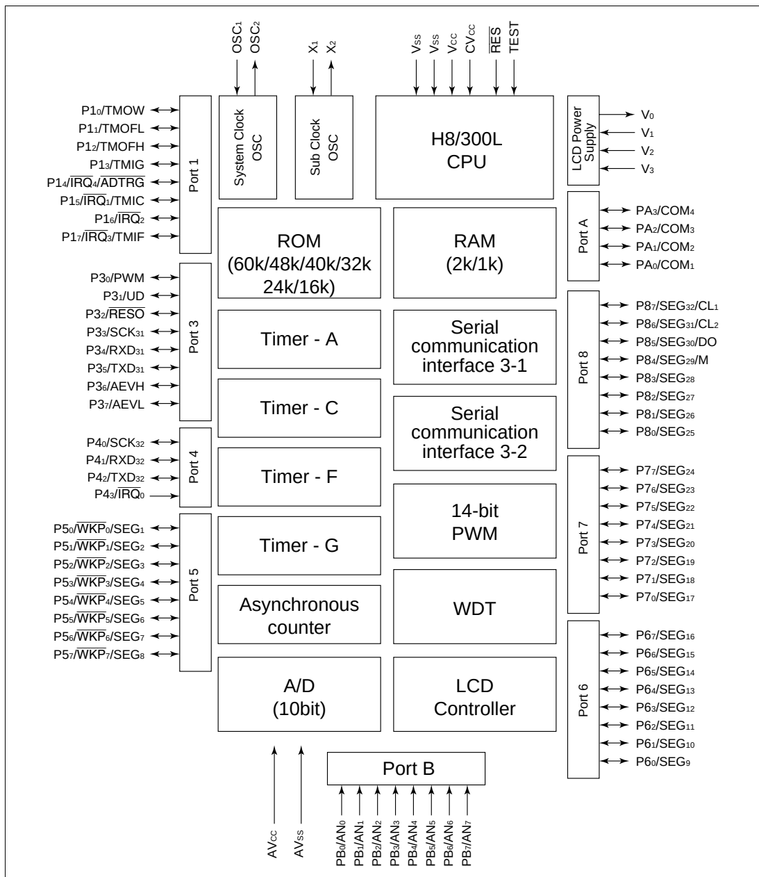
Figure 1.1 Block Diagram
