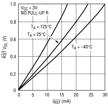
RST V_{OL} vs I_{\text{RST}}
