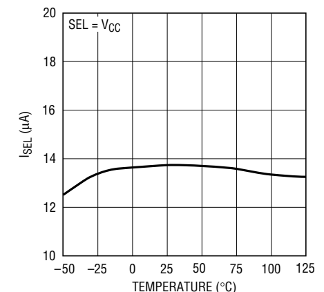
I_{\text{SEL}} vs Temperature
