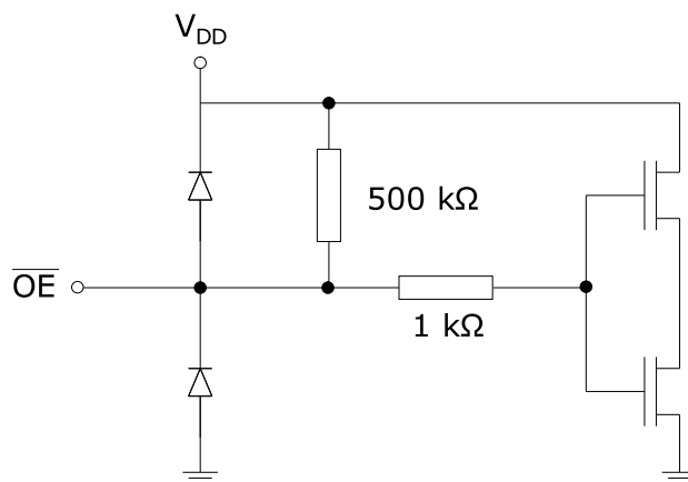
Figure 4. \overline{OE} terminal
