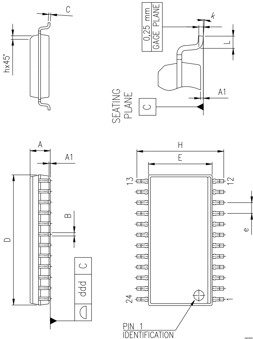
Figure 18. SO-24 package outline
