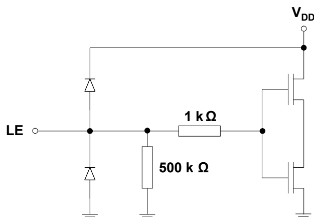
Figure 5. LE terminal
