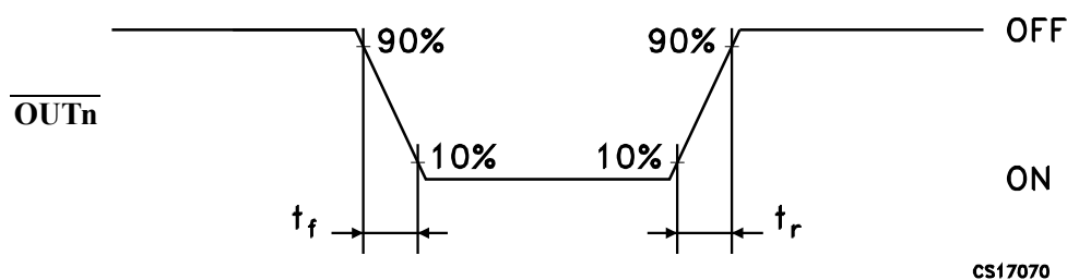
Figure 13. Outputs
