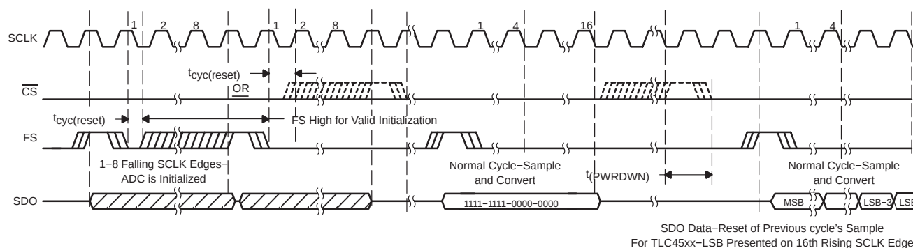
Figure 14. TLC4541/45 Initialization Timing
