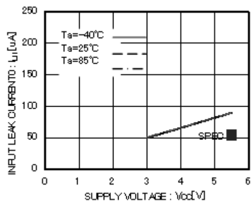
Figure 17. Input Leak Current1 I_{I1} (WPB)
