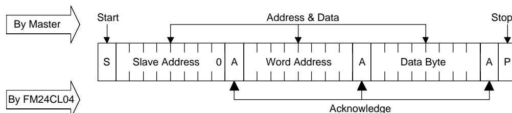
Figure 5. Byte Write
