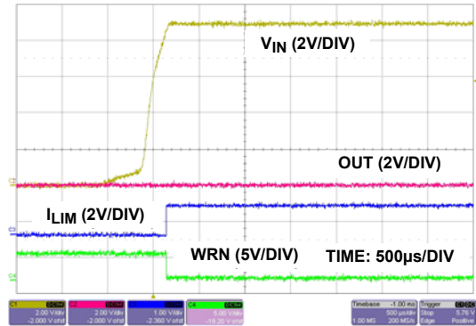
FIGURE 6. TRANSIENT WAVEFORMS WHEN INPUT STEPS FROM ZERO TO 9V
