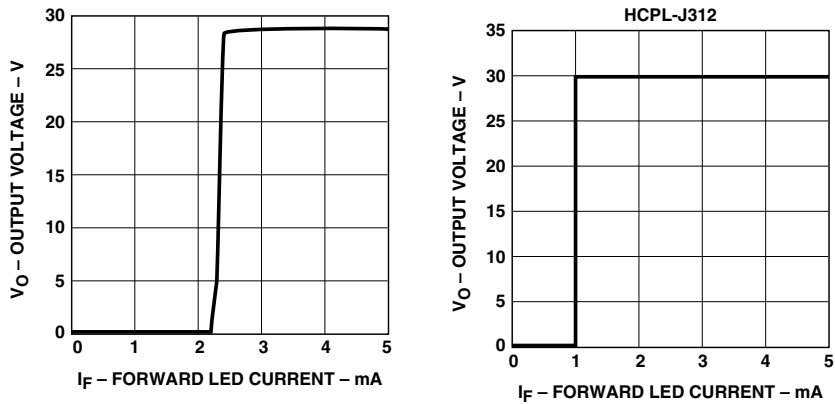
Figure 15. Transfer characteristics.
