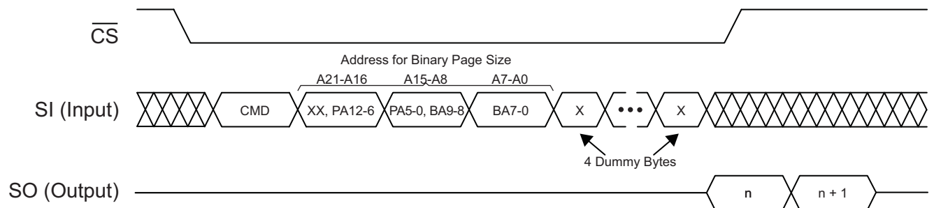
Figure 23-2. Main Memory Page Read
