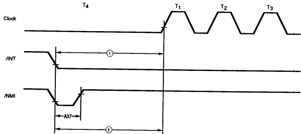
Figure 50. Clock Restart Timing by \overline{INT} , \overline{NMI} (STOP Mode) (See Table B)
