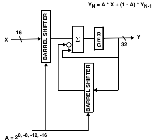
FIGURE 3. LEAKY INTEGRATOR
