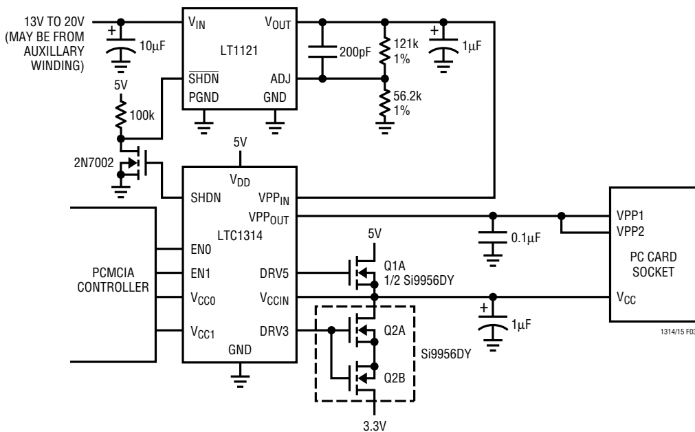
Figure 3. LTC1314 with the LT1121 Linear Regulator
