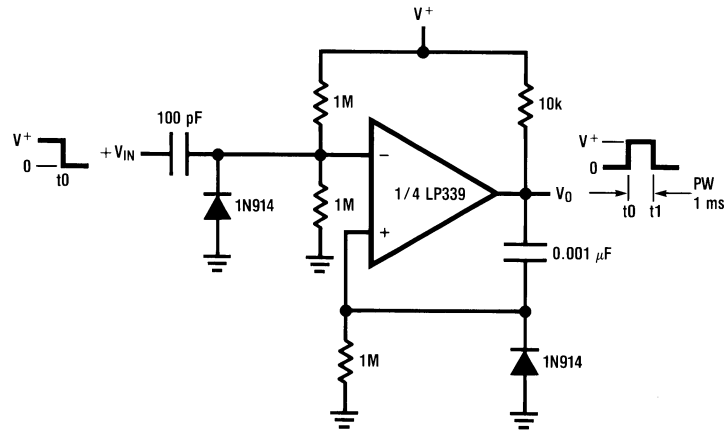
One-Shot Multivibrator
