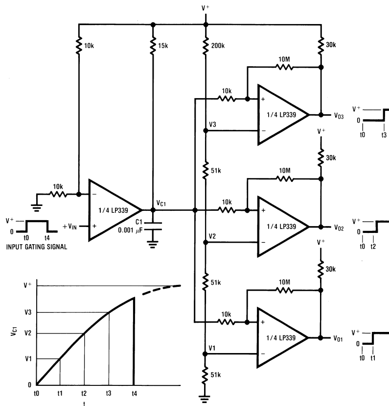
Time-Delay Generator
