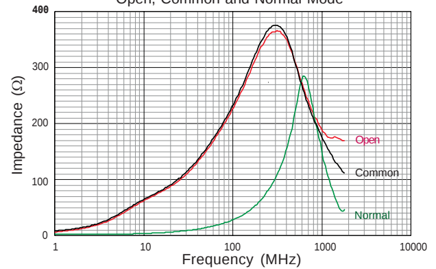
CM3032V221R-00, CM4732V221R-00 & CM6032V221R-00 Z vs. Frequency Open, Common and Normal Mode
