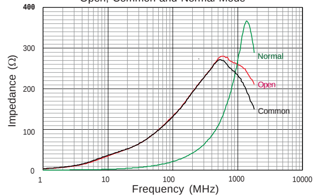
CM3032V131R-00, CM4732V131R-00 & CM6032V131R-00 Z vs. Frequency Open, Common and Normal Mode
