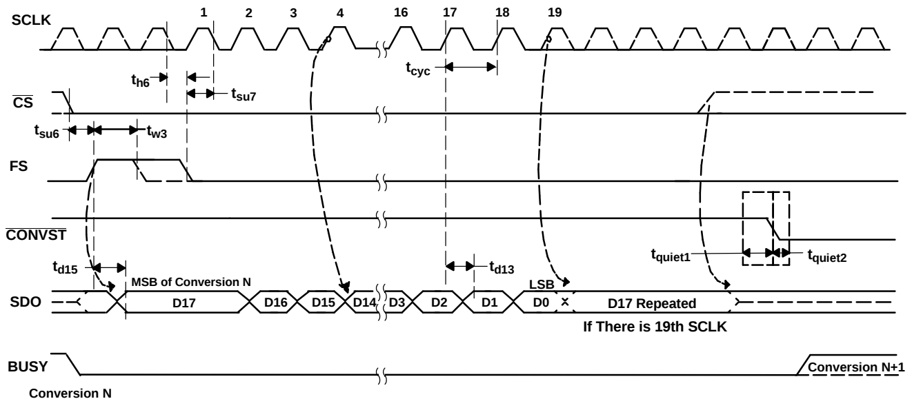
Figure 48. Read Frame Controlled via FS (FS is Low When BUSY Falls)
