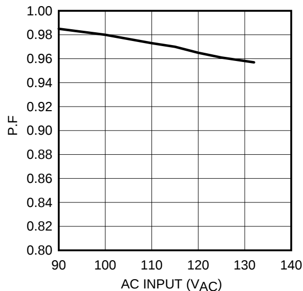
Figure 9. Power Factor
