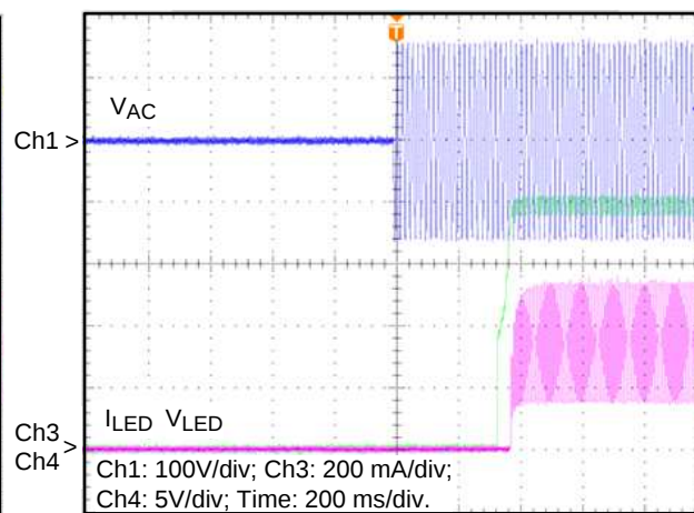
Figure 15. Power Up Output Voltage and Current (120VAC)
