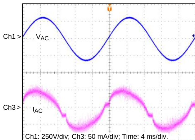
Figure 12. Input Voltage and Input Current (230VAC)
