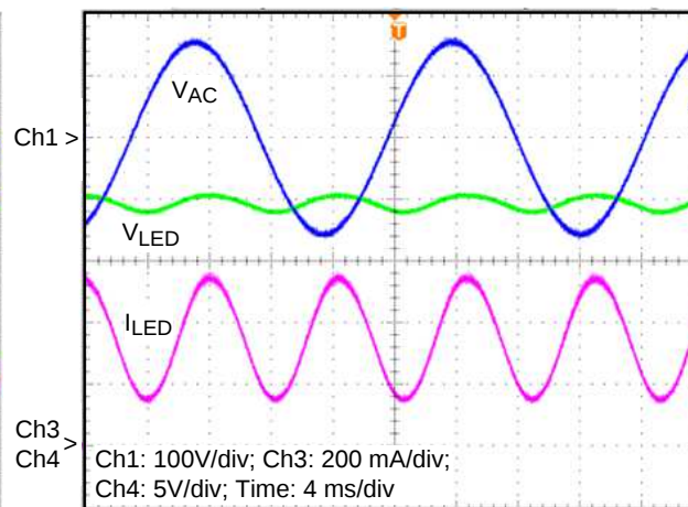
Figure 17. Output Current and Voltage Waveforms (120VAC)
