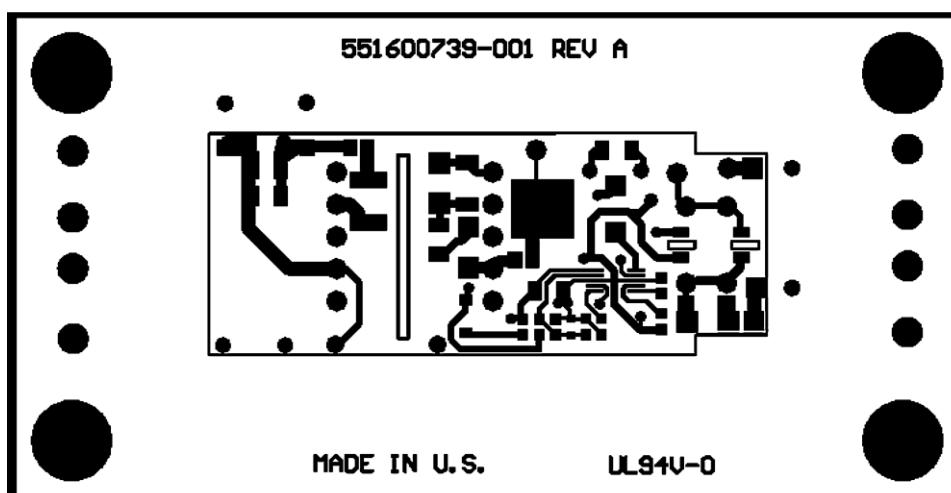
Figure 27. Bottom Layer Copper (Bottom View)
