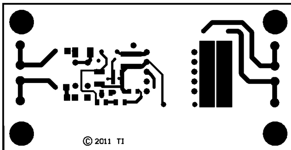
Figure 26. Top Layer Copper (Top View)
