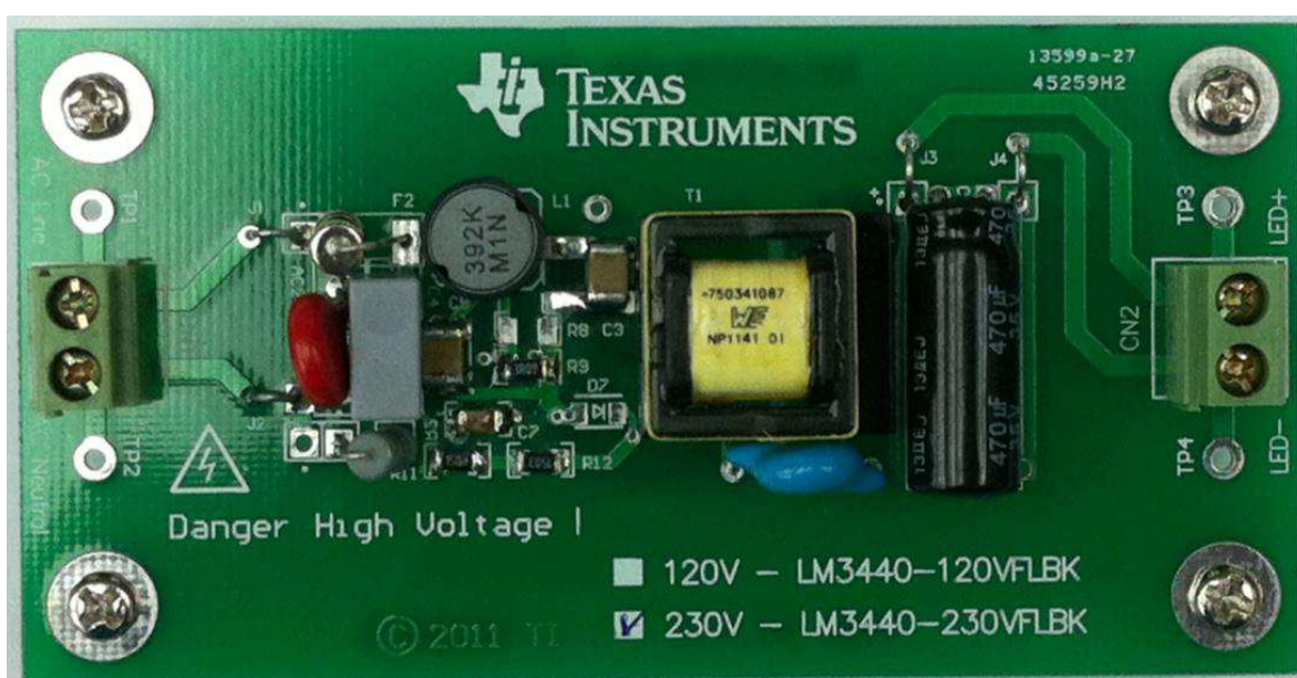
Figure 3. TPS92310EVM_8W
