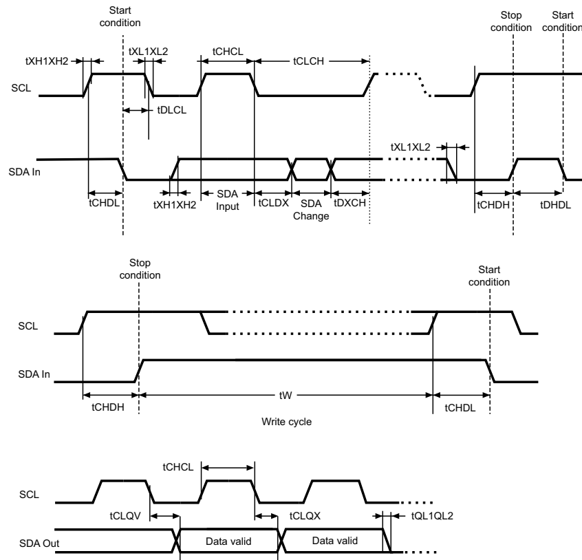
Figure 11. AC waveforms
