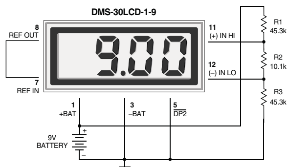
Figure 8. Power Supply Monitor (9V-Powered Models)
