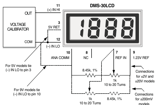
Figure 9. External Gain Adjustment
