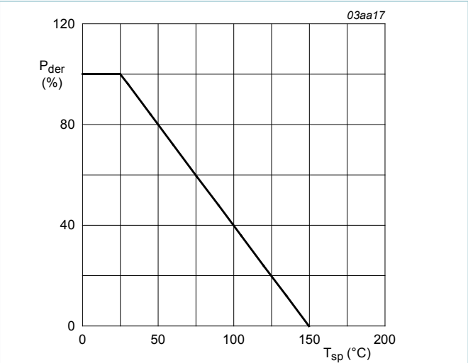
Fig. 2. Normalized total power dissipation as a function of solder point temperature
