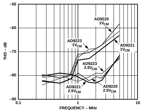
Figure 32a. AD9221/AD9223/AD9220 THD vs. Frequency for V_{CM} = 2.5 \text{ V} and 1.0 \text{ V} ( A_{IN} = -0.5 \text{ dB} , Input Span = 2.0 V p-p)
