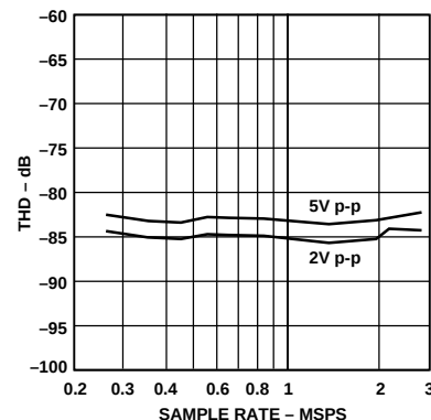
Figure 9. THD vs. Sample Rate ( A_{IN} = -0.5 \text{ dB} , f_{IN} = 500 \text{ kHz} , V_{CM} = 2.5 \text{ V} )
