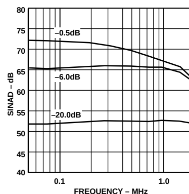
Figure 7. SINAD vs. Input Frequency (Input Span = 5.0 V p-p, V_{CM} = 2.5 \text{ V} )
