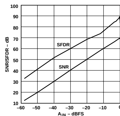
Figure 10. SNR/SFDR vs. A_{IN} (Input Amplitude) ( f_{IN} = 500 \text{ kHz} , Input Span = 2 V p-p, V_{CM} = 2.5 \text{ V} )
