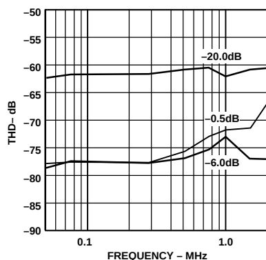
Figure 8. THD vs. Input Frequency (Input Span = 5.0 V p-p, V_{CM} = 2.5 \text{ V} )
