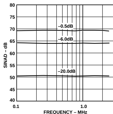
Figure 5. SINAD vs. Input Frequency (Input Span = 2.0 V p-p, V_{CM} = 2.5 \text{ V} )
