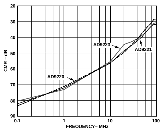
Figure 37. AD9221/AD9223/AD9220 Input CMR vs. Input Frequency
