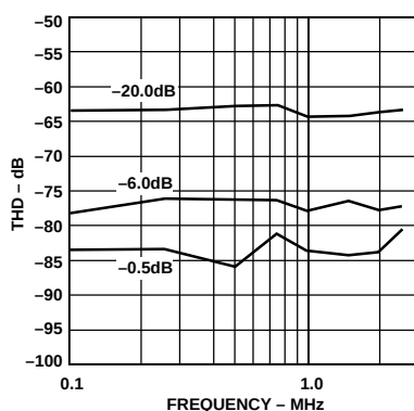
Figure 6. THD vs. Input Frequency (Input Span = 2.0 V p-p, V_{CM} = 2.5 \text{ V} )
