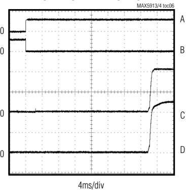
STARTUP WAVEFORMS
