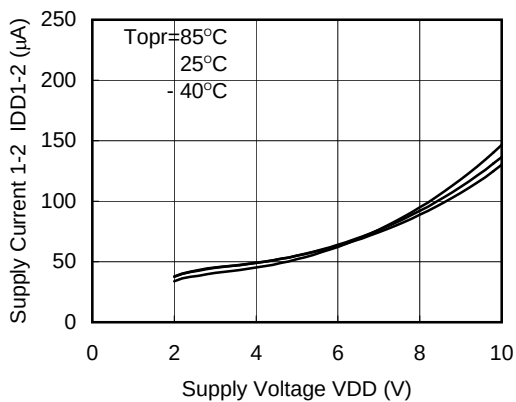
XC9503B092 (180KHz)
