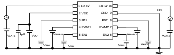
Circuit 6
