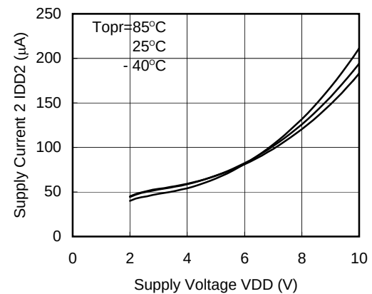
XC9503B092 (180KHz)
