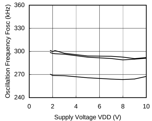
XC9503B093(180kHz)
