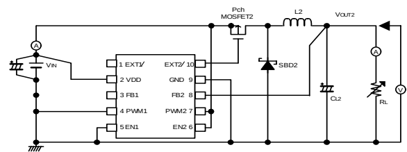
Circuit 7
