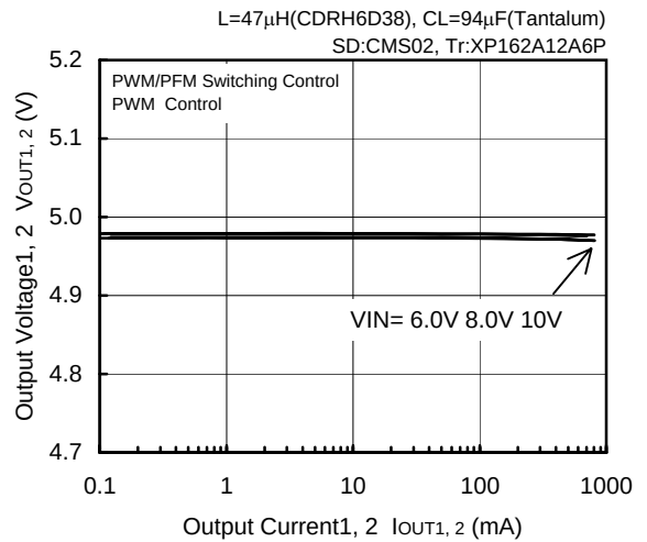
FOSC=180kHz, VOUT1, 2=5.0V
