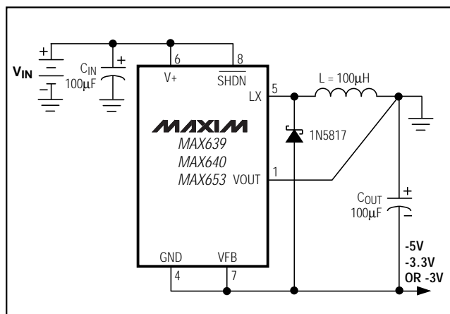
Figure 6. Inverting Configuration
