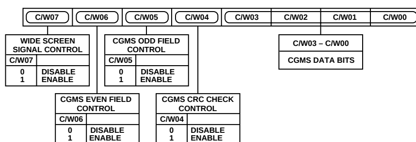
Figure 51. CGMS_WSS Register 0
