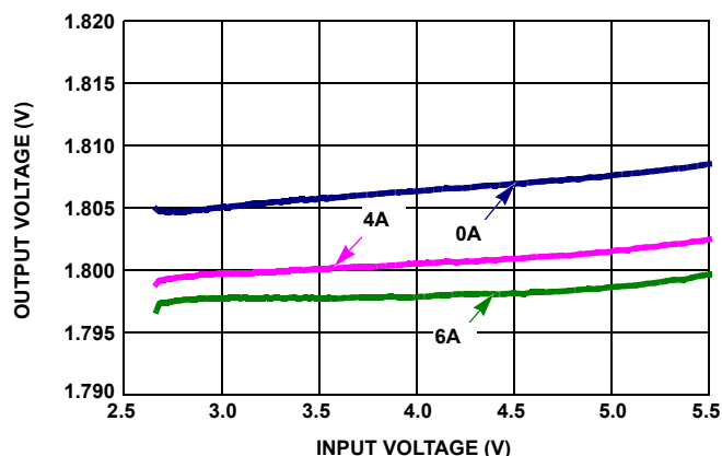
FIGURE 48. OUTPUT VOLTAGE REGULATION vs V_{IN} , T_A = +25^{\circ}C
