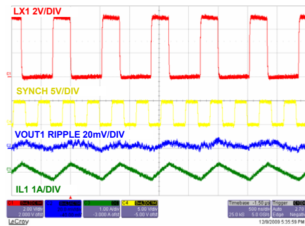
FIGURE 21. STEADY STATE OPERATION CHANNEL 1 AT NO LOAD WITH F_{SW} = 2.4\text{MHz}
