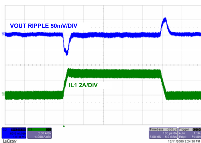
FIGURE 13. LOAD TRANSIENT CHANNEL 1
