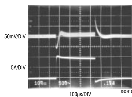
Transient Response
