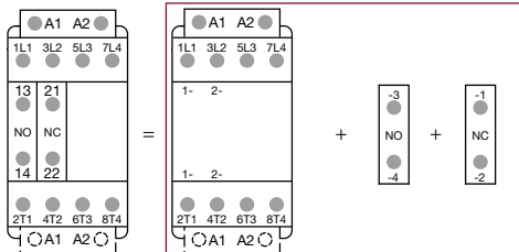
Combination 11 = AF09, AF16..-40-00 + CA4-10 + CA4-01
