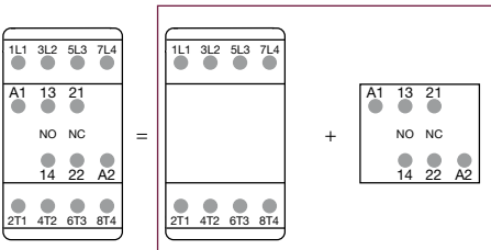
Combination 11 = AF09, AF16..-40-00 + CAT4-11E
