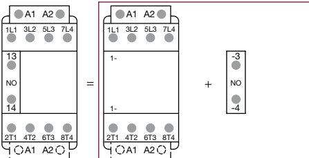
Combination 10 = AF09, AF16..-40-00 + CA4-10
