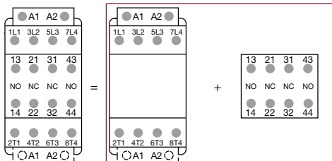
Combination 22 = AF09, AF16..-40-00 + CA4-22E
