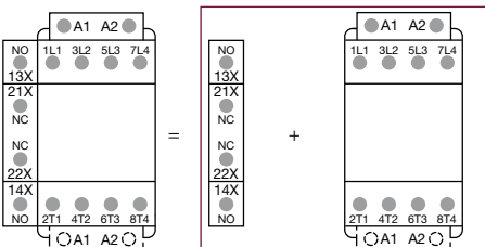
Combination 11 = CAL4-11 + AF09, AF16..-40-00
