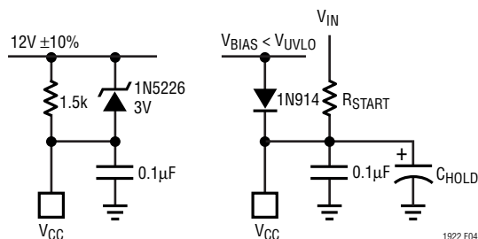
Figure 4. Bias Configurations
