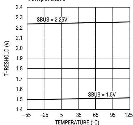
Delay Pin Threshold vs Temperature
