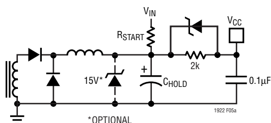
Figure 5a. Auxiliary Winding Bias Supply
