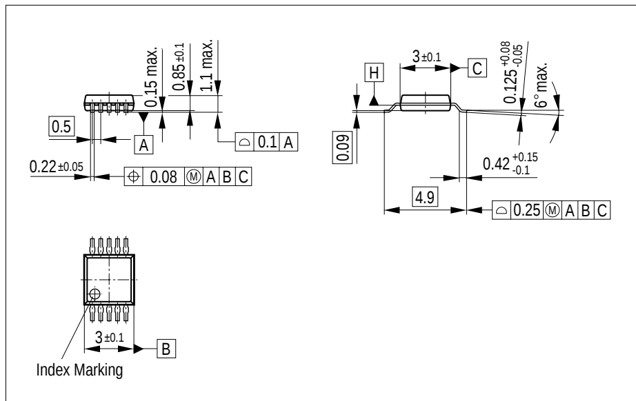
Figure 18 PG-TSSOP-10
