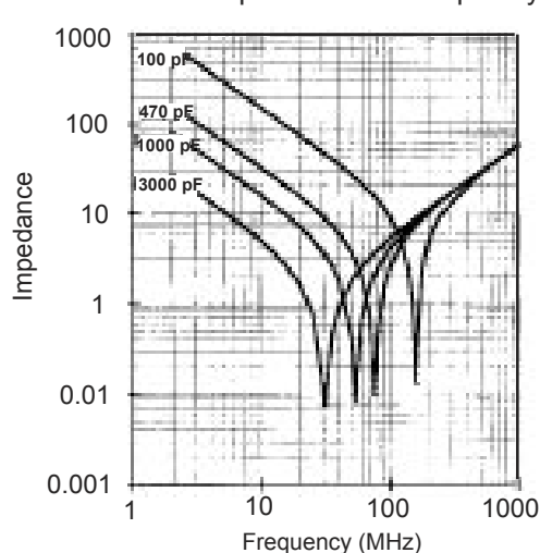
CDV16 Impedance vs. Frequency
