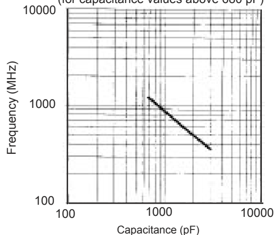
Typical Insertion Loss Notch Frequencies (for capacitance values above 680 pF)
