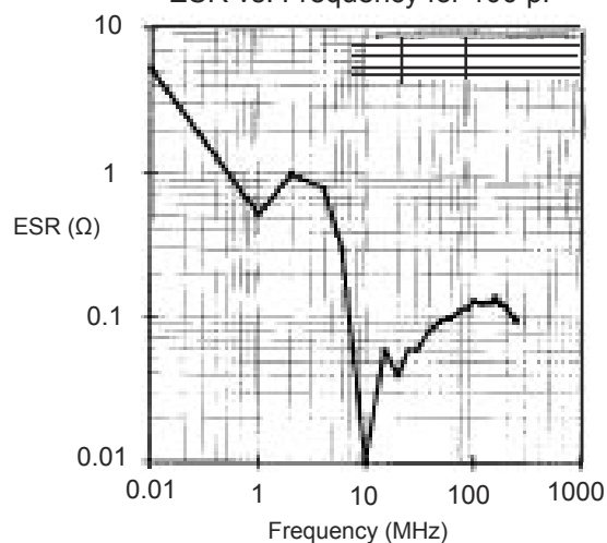
ESR vs. Frequency for 100 pF
