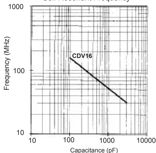
Self Resonant Frequency
