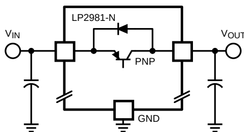
Figure 38. LP2981-N Reverse Current Path
