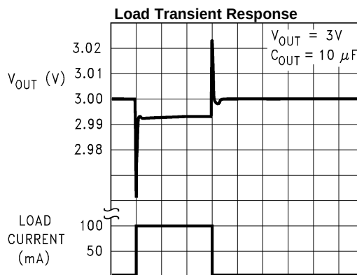
10 \mu\text{s}/\text{div} → Figure 17.
