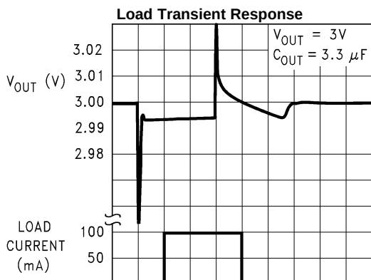
10 \mu\text{s}/\text{div} → Figure 16.
