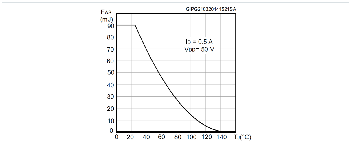
Figure 13. Maximum avalanche energy vs starting T_J
