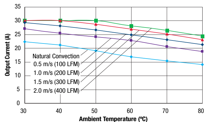
UCE-3.3/30-D48 Maximum Current Temperature Derating (Vin=48V, no baseplate, transverse airflow at sea level)
