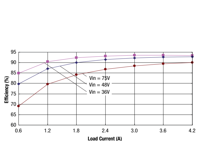
UCE-12/4.2-D48 Efficiency Vs. Line Voltage & Load Current @ +25°C
