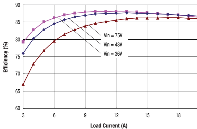
UCE-1.8/30-D48 Efficiency vs Line Voltage & Load Current @ 25°C
