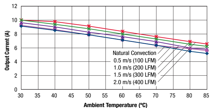
UCE-12/10-D48 Maximum Current Temperature Derating at sea level (Vin = 48V, no baseplate, airflow direction from Vin to Vout)
