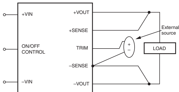
Figure 5. Trimming with an external source
