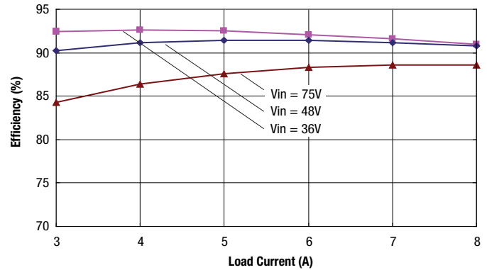
UCE-12/8.3-D48 Efficiency vs Line Voltage & Load Current @ 25°C
