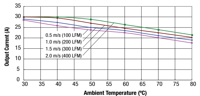
UCE-1.8/30-D48 Maximum Current Temperature Derating (Vin = 48V, no baseplate, longitudinal airflow at sea level)
