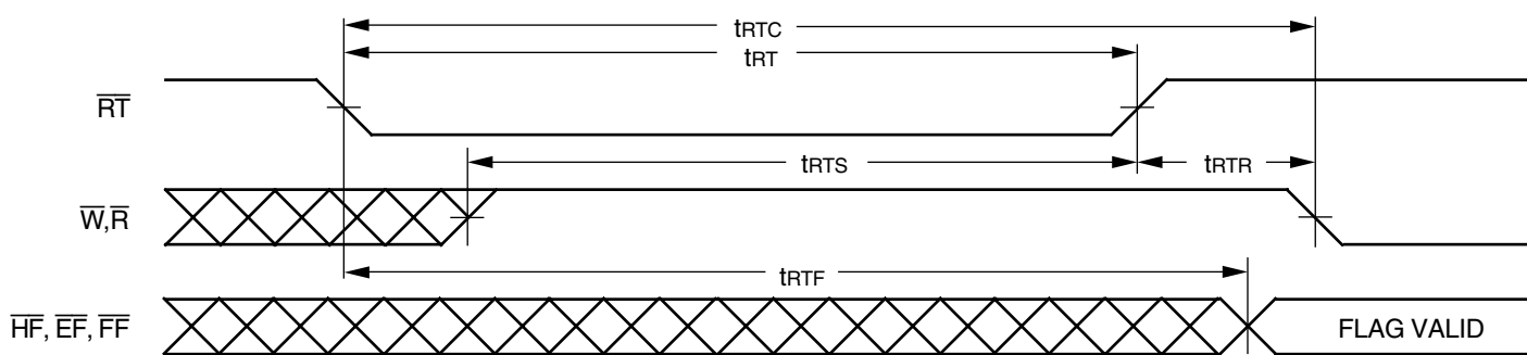
Figure 6. Retransmit
