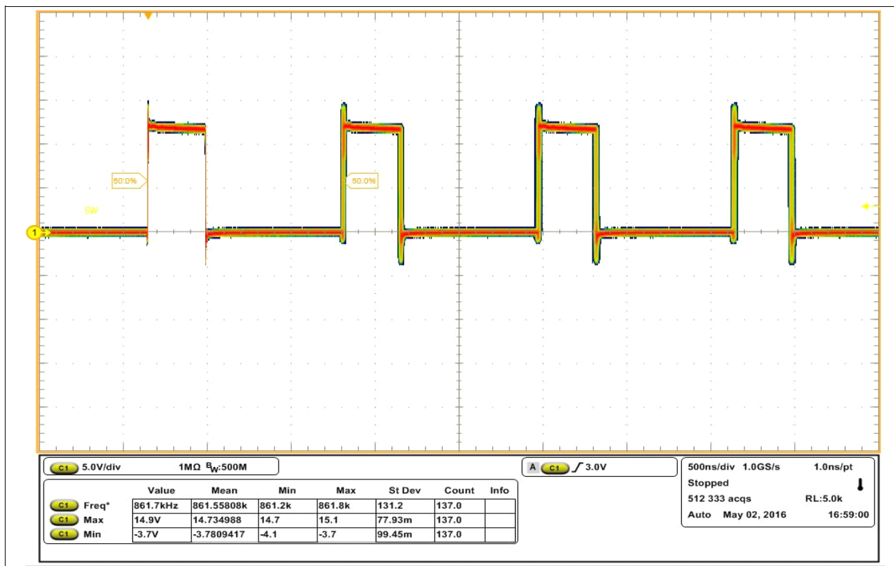
Figure 7-6 FCCM, SW node, 3A
