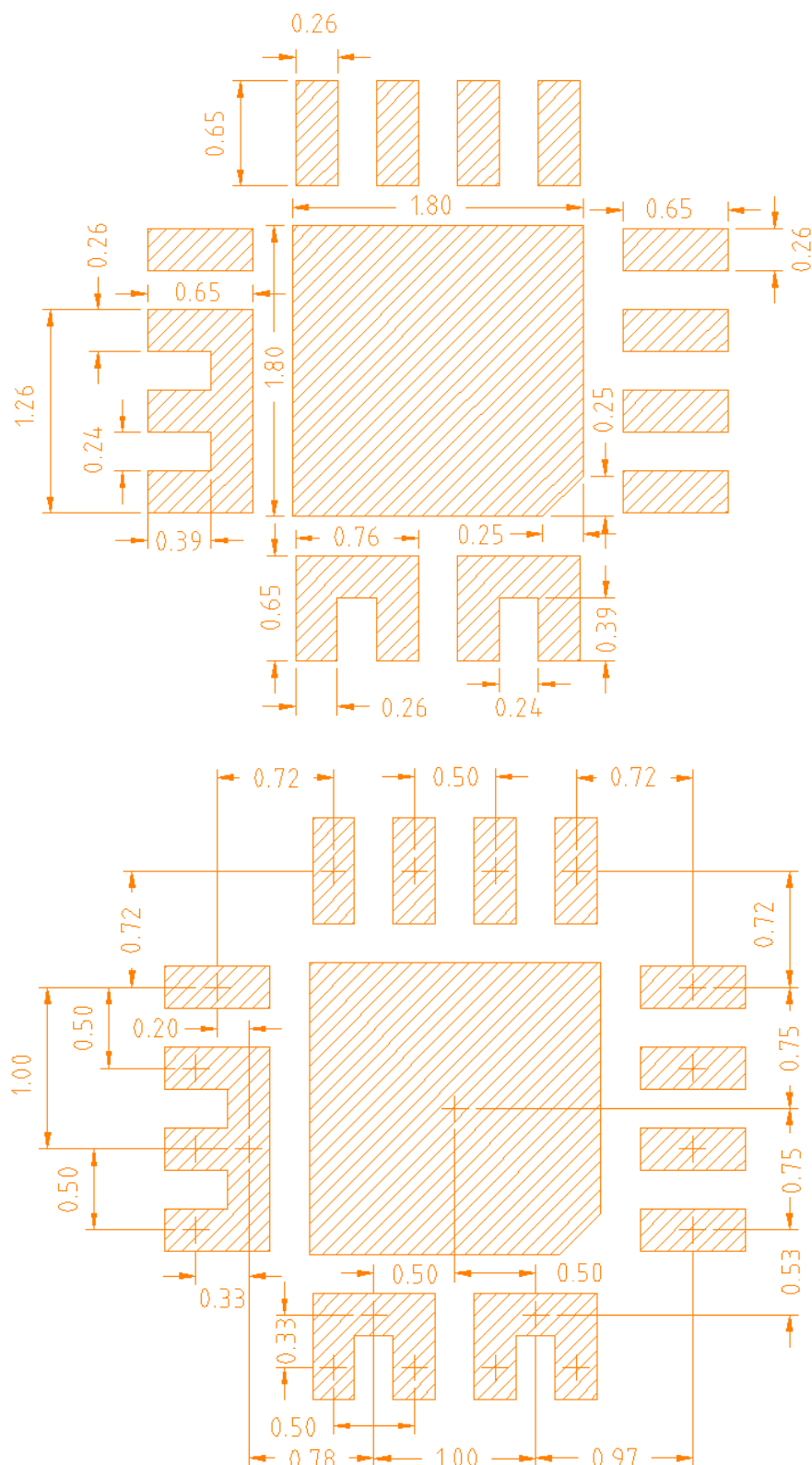
Figure 8-5 PCB metal pad sizing and spacing (all dimensions in mm)
