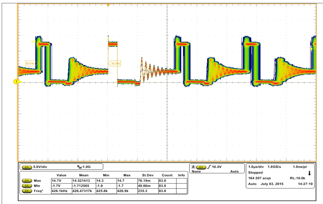
Figure 7-7 Diode Emulation Mode, SW node, 0.3A
