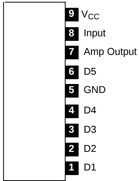
Pin Connection Diagram (Front View)
