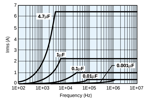
100 VDC / 63 VAC
