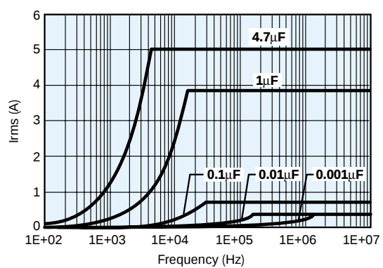
100 VDC / 63 VAC
