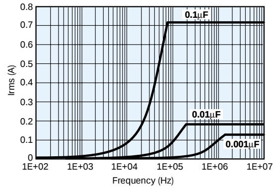
25 VDC / 15 VAC
