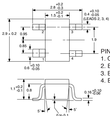
PACKAGE OUTLINE 39R
