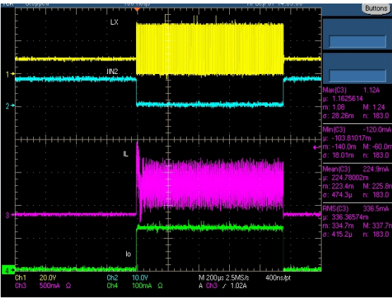
FIGURE 9. LX, VIN, IL AND IO AT PWM DIMMING (54 LEDs, 20mA, V_{IN} = 12V )
