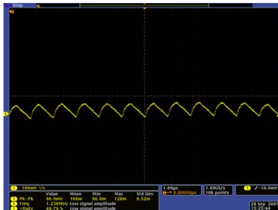
FIGURE 16. RIPPLE VOLTAGE ZOOM IN (54 LEDs, V_{IN} = 12V , 20mA EACH, C_{OUT} = 4 \times 4.7\mu F/50V )
