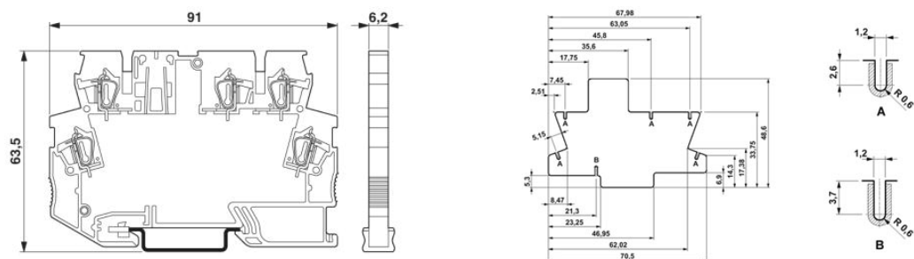
Dimensional drawing of the PCB Elongated holes (detail A and B) must be through-plated in the hatched section
