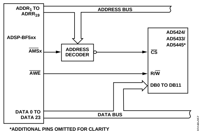
Figure 58. ADSP-BF5xx-to-AD5424/AD5433/AD5445 Interface
