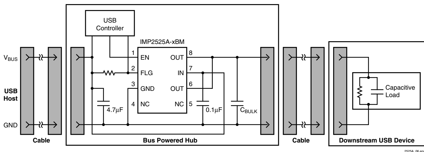
Figure 2. Soft-Start Application
