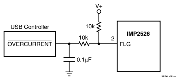
Figure 4. Transient Filter
