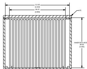
SECTION C-C SCALE 3 / 4
