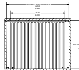
SECTION D-D SCALE 3 / 4
