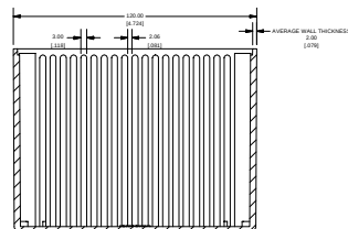
SECTION A-A SCALE 3 / 4
