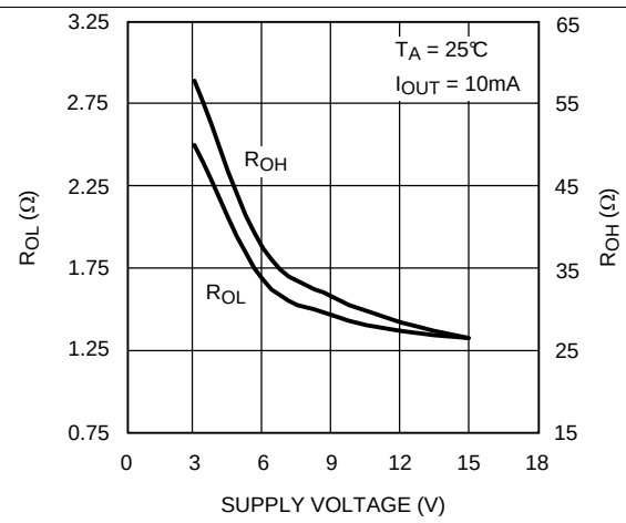
Figure 10. R_{DS(on)} vs Supply Voltage
